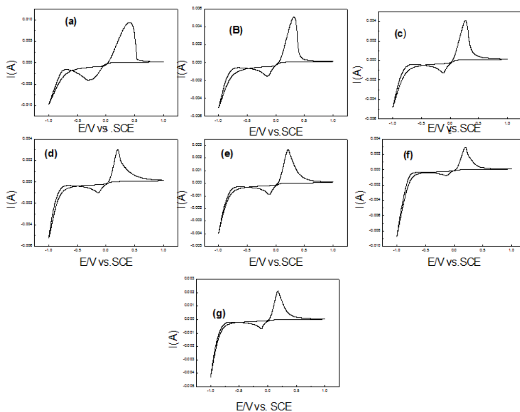
Figure 3. Cyclic voltammetry of Cu-Ni mixed solution after each deposition, from (a) to (g) respectively correspond to samples number used during the deposition process at scan rate 50mv/s
