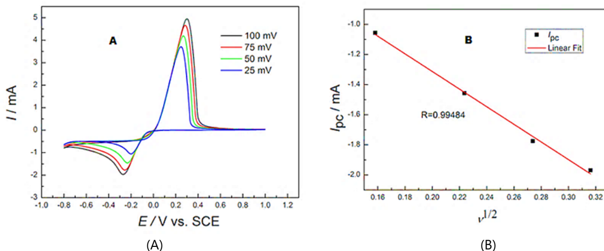
Figure 4. (A) Cyclic voltammetry of 6.392 g/l of CuSO 4 at the graphite electrode using different scan rates. (B) Graph of cathodic peak vs the square root of the scan rate
