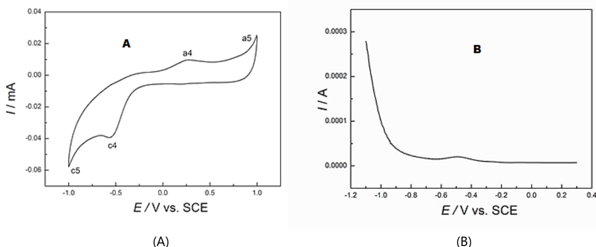
Figure 6. (A) Cyclic voltammetry curve of 1.766 g/l of NiSO 4 solution at 100mv/s. (B) linear sweep voltammetry of 1.766 g/l of NiSO 4 solution at 100mv/s
