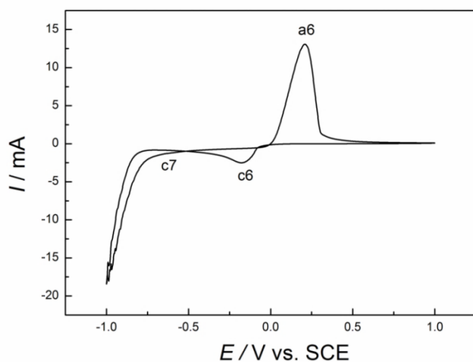
Figure 7. Cyclic voltammetry of 6.392 g/l of \text{CuSO}_4 and 2.944 g/l of \text{NiSO}_4 mixed solution at 100mv/s
