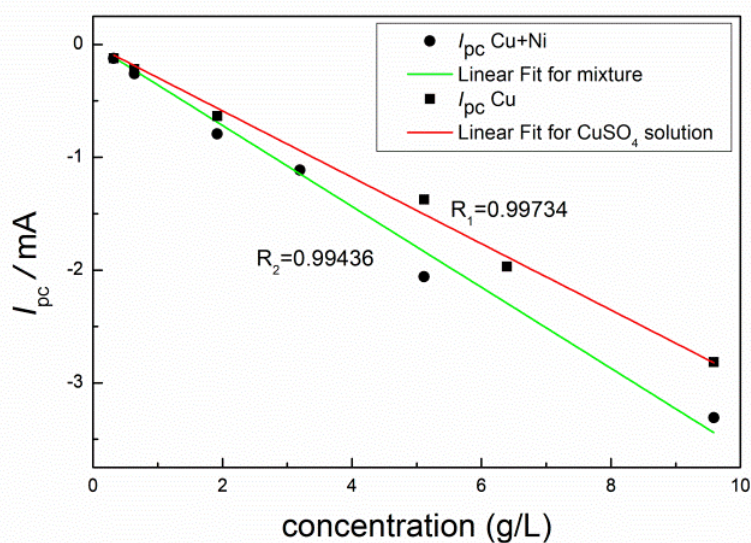
Figure 10. Comparison of linear fit of current cathodic potential peak in function of copper concentration in Cu-Ni mixed solution and copper solution
