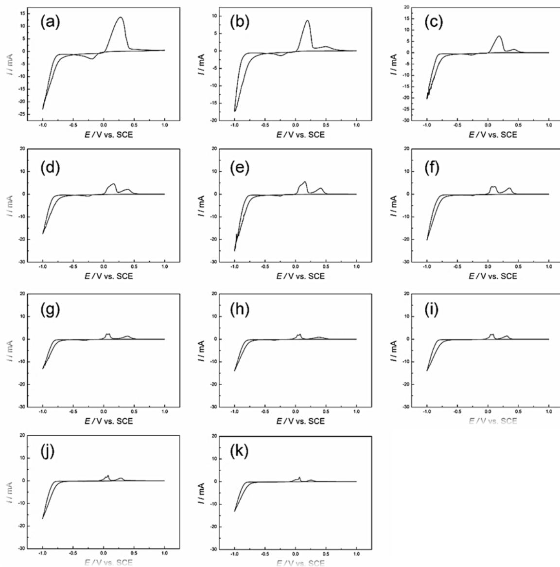
Figure 16 (continued). Cyclic voltammetry of Cu-Ni mixed solution after each deposition, from (a) to (k) respectively correspond to samples number used during the deposition process at scan rate 50mv/s
