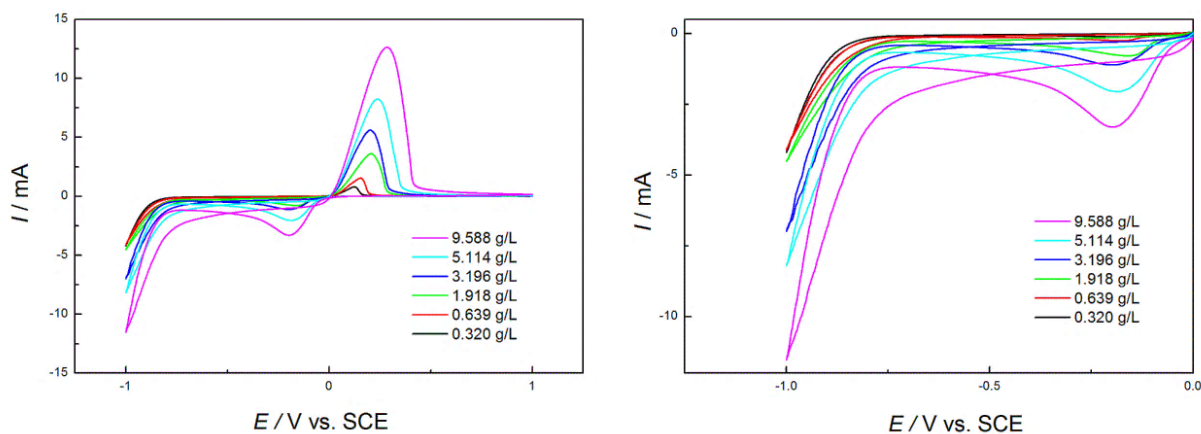
Figure 9. Cyclic voltammetry of different concentrations of \text{CuSO}_4 and 2.944 g/l of \text{NiSO}_4 in Cu-Ni mixed solution at 100mv/s
