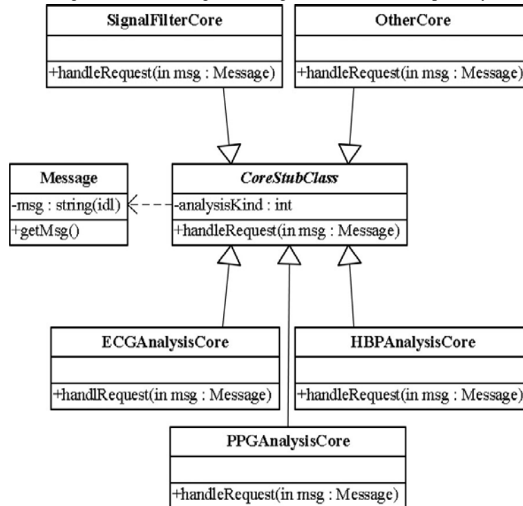
Fig. 3: Plug-in algorithm framework
