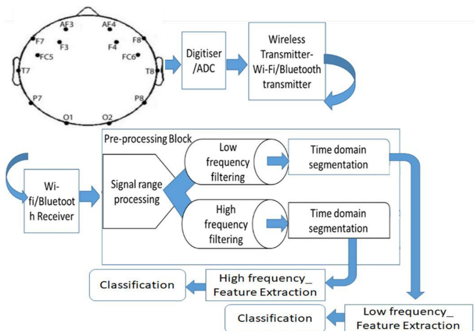
Fig 1: Block diagram of our set-up for emotion analysis with lobe-based activity based on strength of the signals in high and low frequency band (HFB and LFB)
